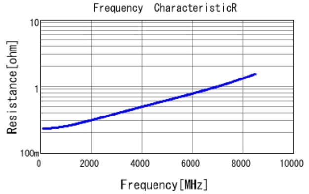
GRM0335C1H4R1BA01 R DCOV, 25degC
