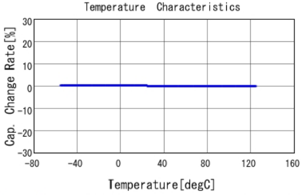
GRM0335C1H4R1BA01 C-Temp. capchange, DCOV, AC1Vrms
