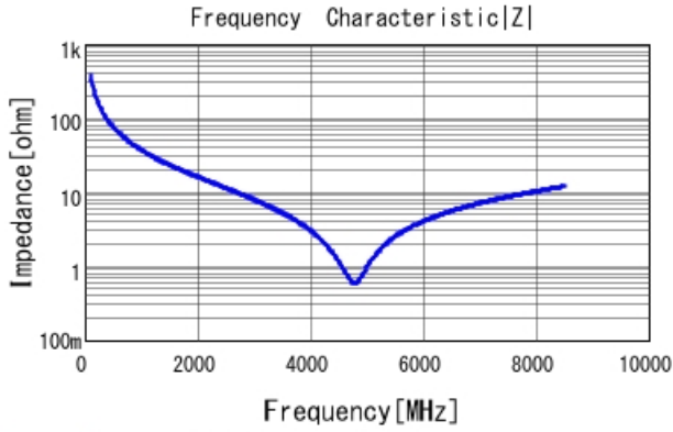
GRM0335C1H4R1BA01 |Z| DCOV, 25degC
