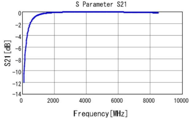
GRM0335C1H4R1BA01 S21 DCOV, 25degC
