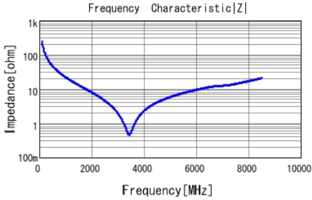
GRM1555C2A6R6CA01 |Z| DCOV, 25degC
