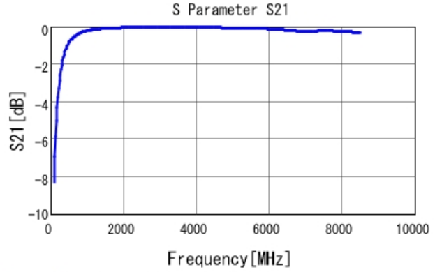
GRM1555C2A6R6CA01 S21 DCOV, 25degC
