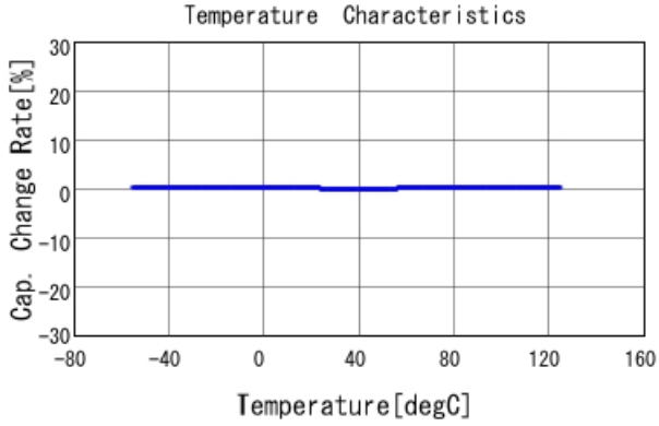
GRM1555C2A6R6CA01 C-Temp. capchange, DCOV, AC1Vrms
