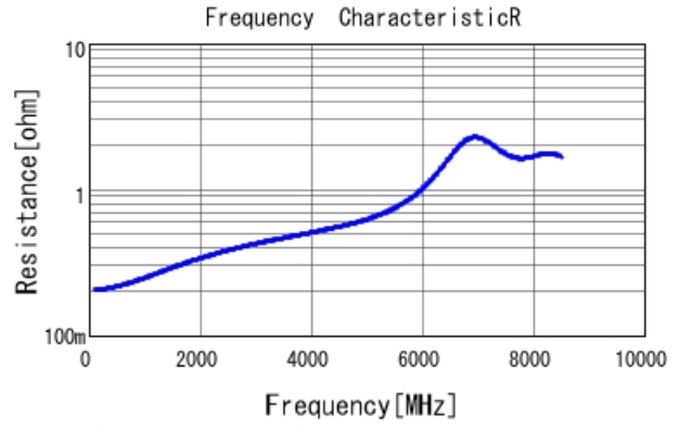
GRM1555C2A6R6CA01 R DCOV, 25degC
