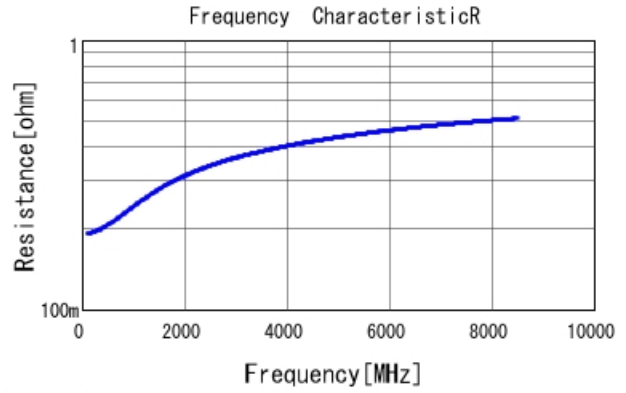
GRM0225C1E3R3CA03 R DCOV, 25degC
