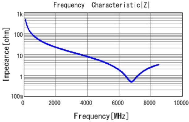
GRM0225C1E3R3CA03 |Z| DCOV, 25degC
