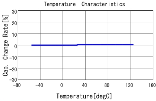
GRM0225C1E3R3CA03 C-Temp. capchange, DC0V, AC1Vrms
