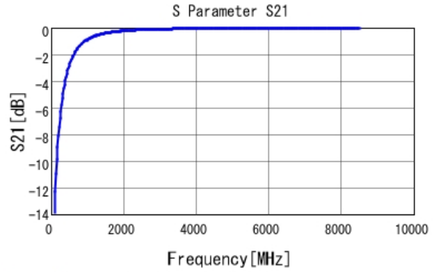
GRM0225C1E3R3CA03 S21 DC0V, 25degC
