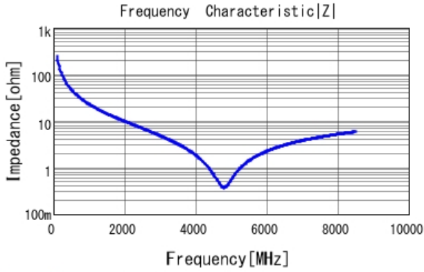
GRM0225C1E6R6BA03 |Z| DCOV, 25degC
