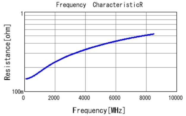
GRM0225C1E6R6BA03 R DCOV, 25degC
