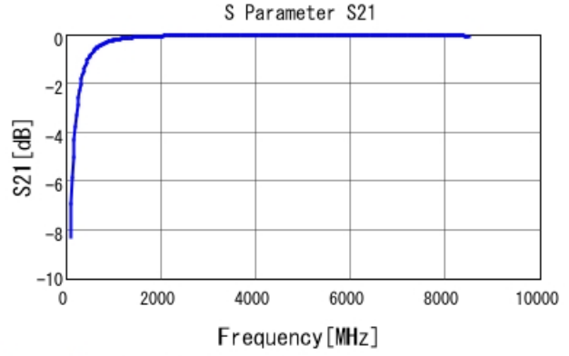
GRM0225C1E6R6BA03 S21 DCOV, 25degC
