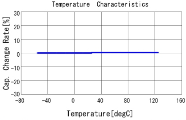
GRM0225C1E6R6BA03 C-Temp. capchange, DCOV, AC1Vrms
