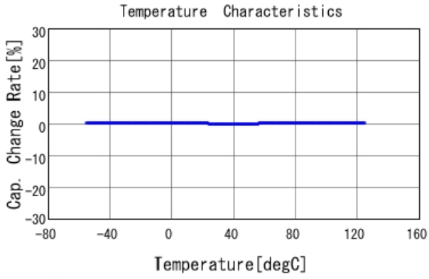
GRM1555C2A7R2WA01 C-Temp. capchange, DCOV, AC1Vrms
