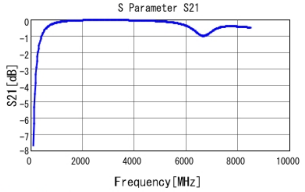
GRM1555C2A7R2WA01 S21 DCOV, 25degC
