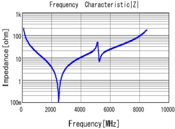
■ GQM2195C2A8R0DB01 |Z| DC0V, 25degC
