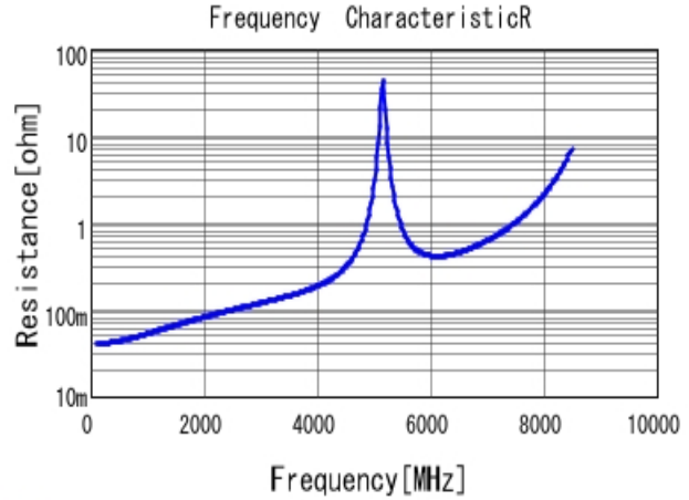
■ GQM2195C2A8R0DB01 R DC0V, 25degC
