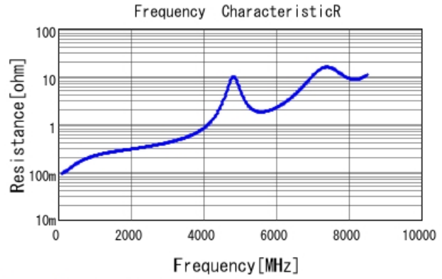
GRM1885C1H9R7CA01 R DCOV, 25degC
