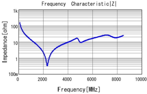
GRM1885C1H9R7CA01 |Z| DCOV, 25degC
