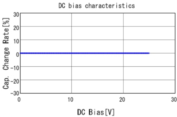
GCM0335C1E5R0CA16 C-DC bias capchange, 25.0degC, AC1V
