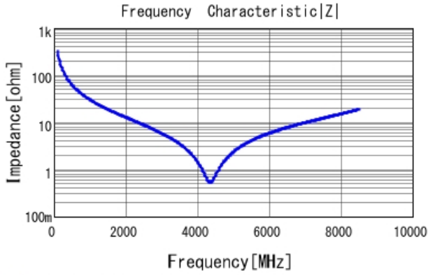
GCM0335C1E5R0CA16 |Z| DCOV, 25degC
