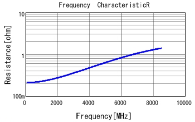
GCM0335C1E5R0CA16 R DCOV, 25degC
