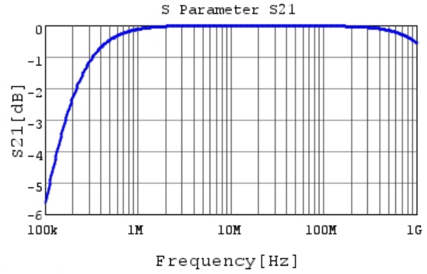
RDED72J103K2M1H03A S21 DCOV, 25degC
