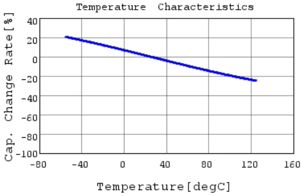
RDED72J103K2M1H03A C-Temp. capchange, DCOV,
