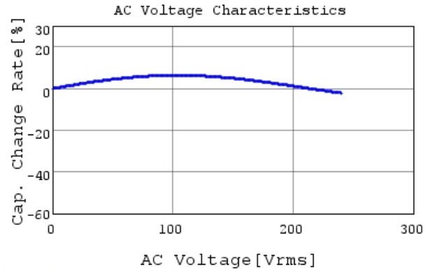
RDED72J103K2M1H03A C-AC Voltage capchange, I
