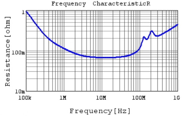
RDED72J103K2M1H03A R DCOV,25degC
