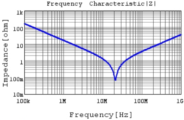
RDED72J103K2M1H03A |Z| DCOV,25degC
