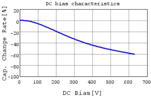
RDED72J103K2M1H03A C-DC bias capchange, 25.0
