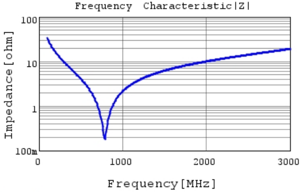
GRM31A5C3A470GW01 |Z| DC0V, 25degC
