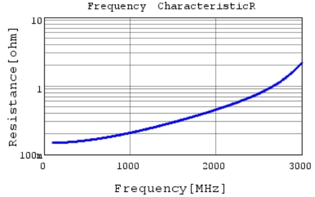
GRM31A5C3A470GW01 R DC0V, 25degC
