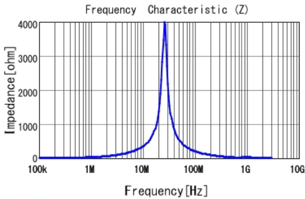
DFE252012F-4R7M |Z|
