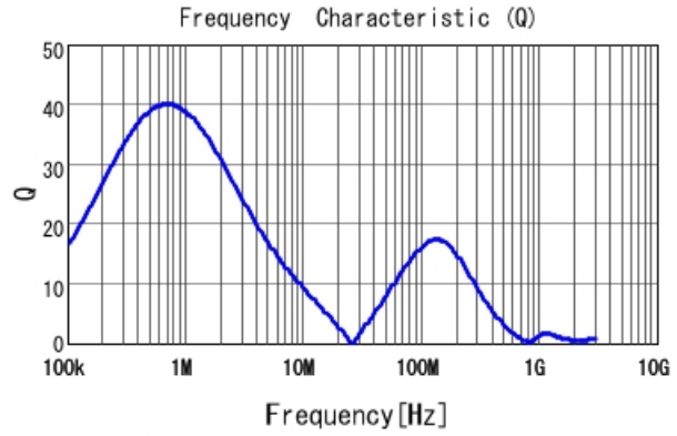
DFE252012F-4R7M Q
