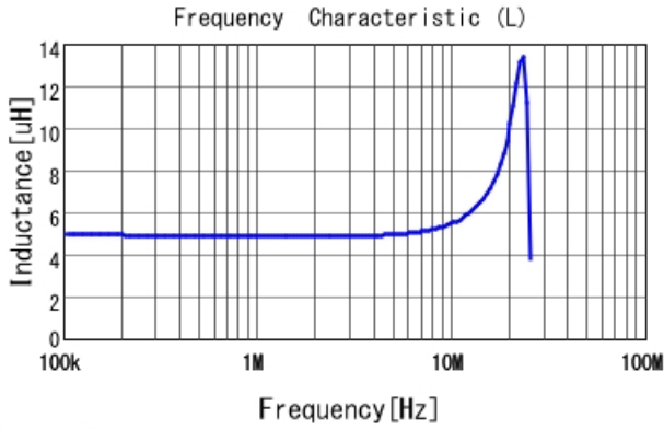
DFE252012F-4R7M L
