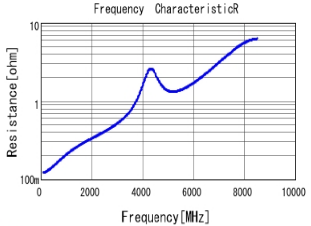
■ GRM1555C2A180GA01 R DC0V, 25degC
