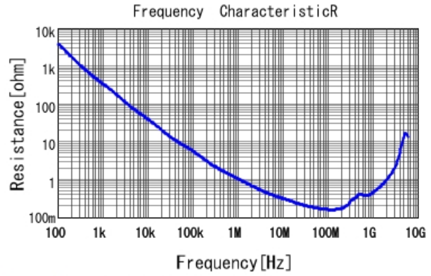
GRM188R71E222KA01 R DCOV, 25degC
