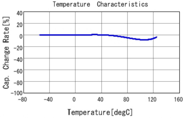
GRM188R71E222KA01 C-Temp. capchange, DC0.0V, AC1.C
