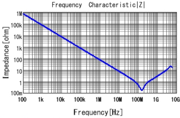
GRM188R71E222KA01 |Z| DCOV, 25degC
