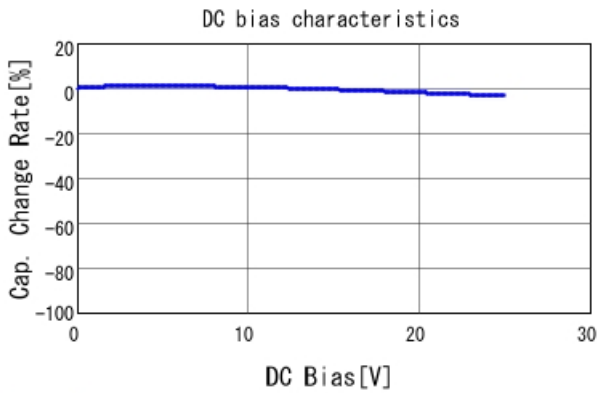
GRM188R71E222KA01 C-DC bias capchange, 25.0degC, A
