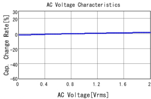
GRM188R71E222KA01 C-AC Voltage capchange, DCOV, 25
