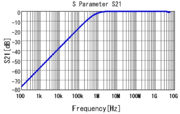
GRM188R71E222KA01 S21 DC0V, 25degC
