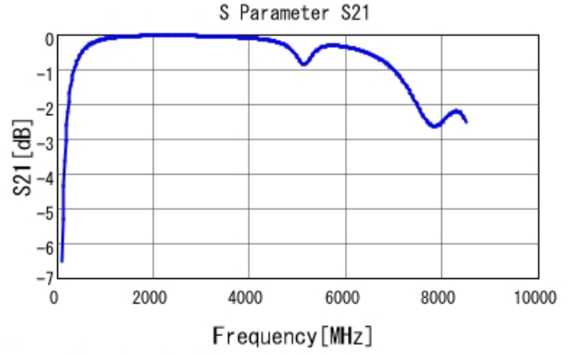
GRM1885C1H8R5WA01 S21 DCOV, 25degC
