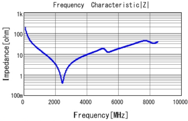
GRM1885C1H8R5WA01 |Z| DCOV, 25degC
