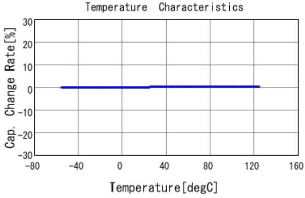
GRM1885C1H8R5WA01 C-Temp. capchange, DCOV, AC1Vrms
