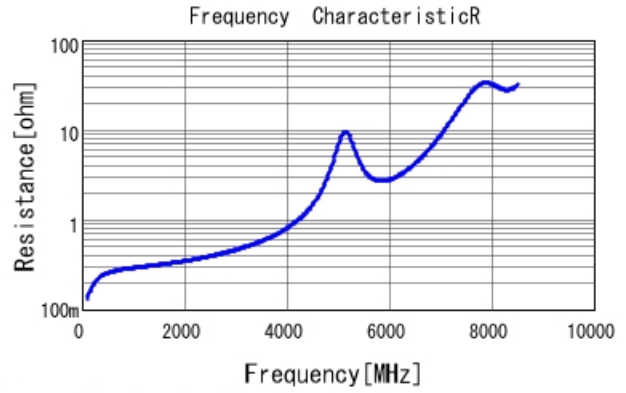
GRM1885C1H8R5WA01 R DCOV, 25degC
