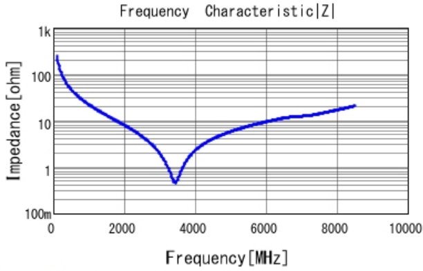
GRM1555C2A6R6BA01 |Z| DCOV, 25degC
