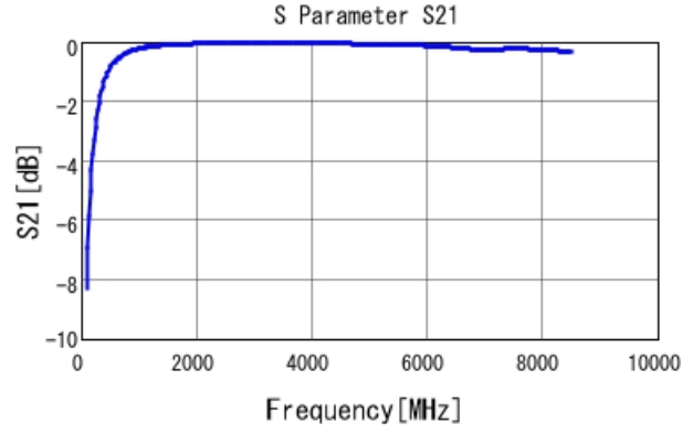
GRM1555C2A6R6BA01 S21 DCOV, 25degC
