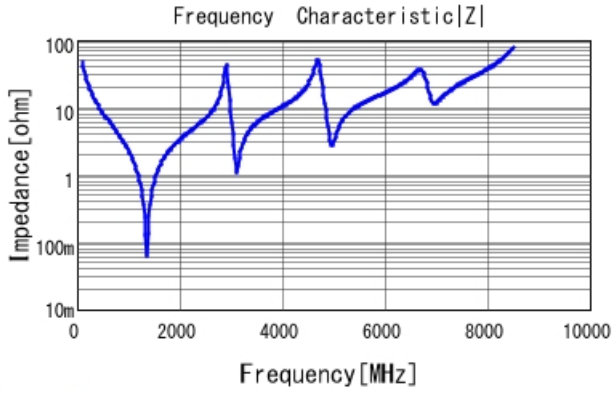
GQM2195C2E330JB12 |Z| DCOV, 25degC
