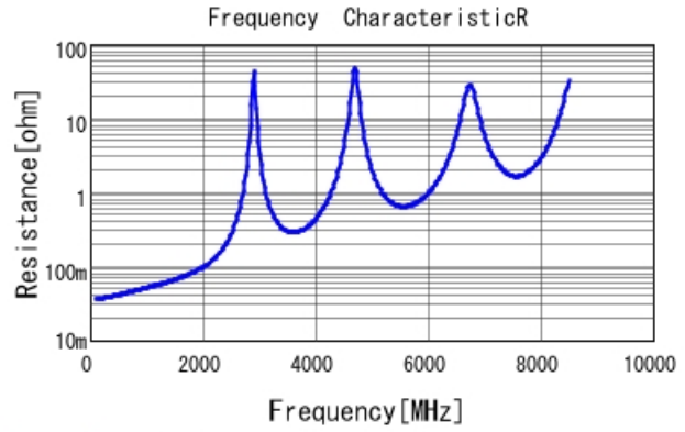
GQM2195C2E330JB12 R DCOV, 25degC
