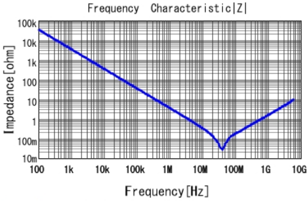
GGM155R71C473KA37 |Z| DCOV, 25degC
