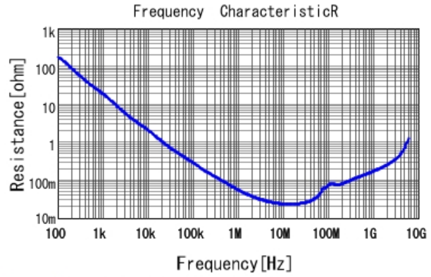
GGM155R71C473KA37 R DCOV, 25degC
