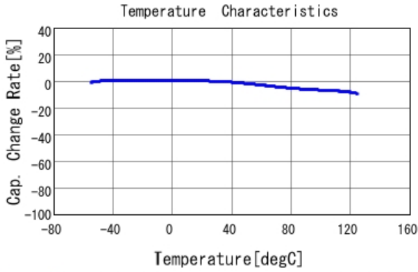
GGM155R71C473KA37 C-Temp. capchange, DC0.0V, AC1.C
