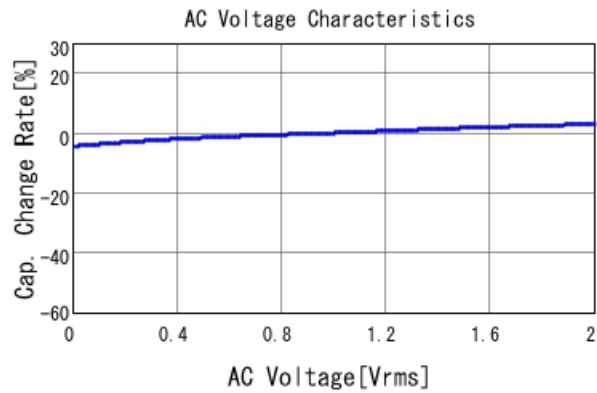
GGM155R71C473KA37 C-AC Voltage capchange, DCOV, 25
