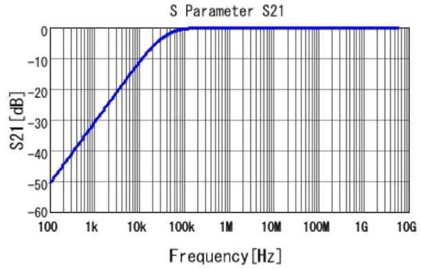
GGM155R71C473KA37 S21 DC0V, 25degC
