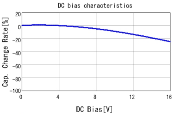
GGM155R71C473KA37 C-DC bias capchange, 25.0degC, A
