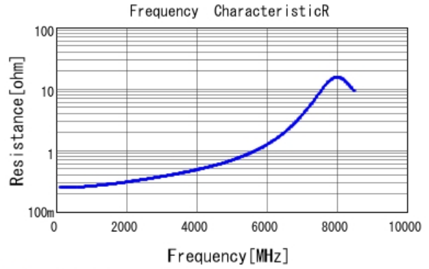
GCM1555C1H4R7CA16 R DC0V, 25degC
