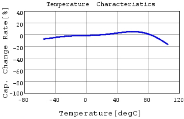
GRT31CC81E106KE01 C-Temp. capchange, DC0.0V,
