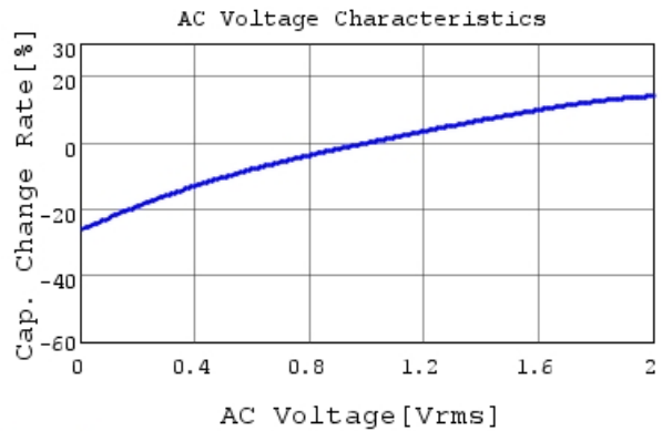
GRT31CC81E106KE01 C-AC Voltage capchange, Dc
