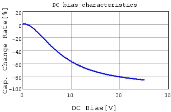
GRT31CC81E106KE01 C-DC bias capchange, 25.0c
