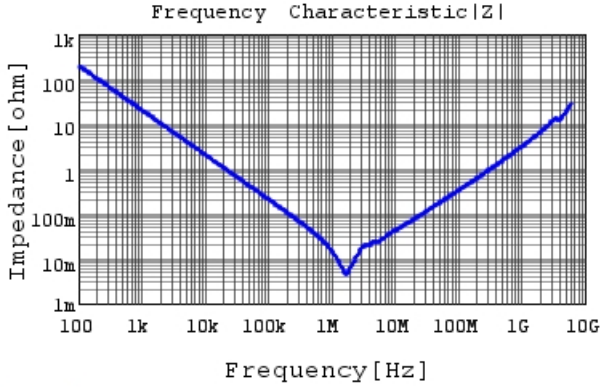
GRT31CC81E106KE01 |Z| DCOV, 25degC
