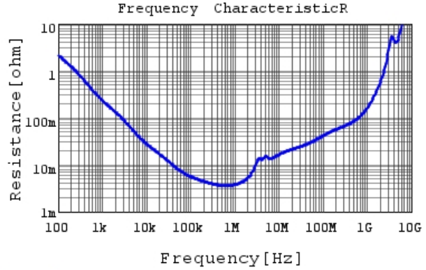
GRT31CC81E106KE01 R DCOV, 25degC
