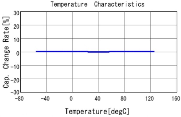
GRM1555C1H4R8BA01 C-Temp. capchange, DC0V, AC1Vrms
