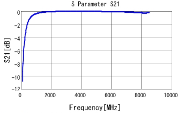
GRM1555C1H4R8BA01 S21 DC0V, 25degC
