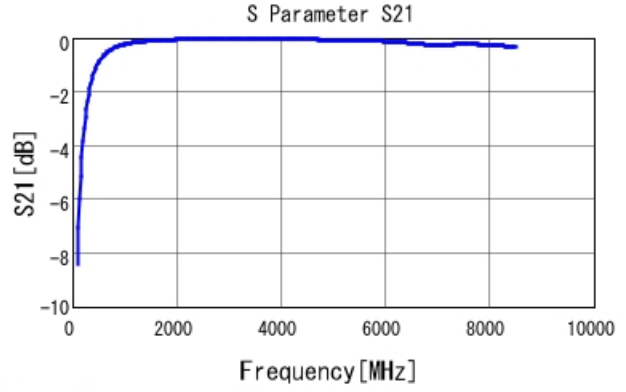
GRM1555C2A6R5WA01 S21 DCOV, 25degC
