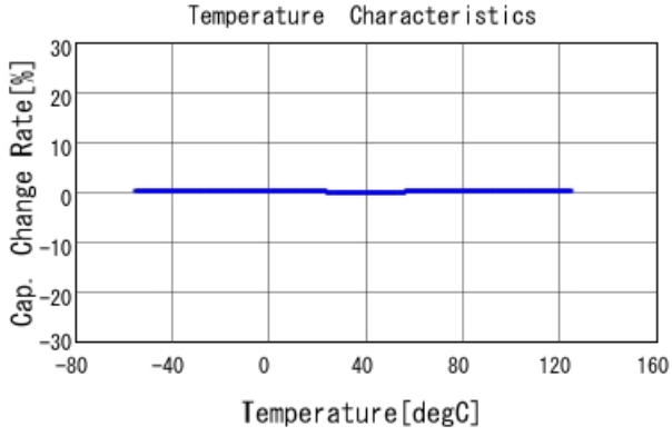
GRM1555C2A6R5WA01 C-Temp. capchange, DCOV, AC1Vrms
