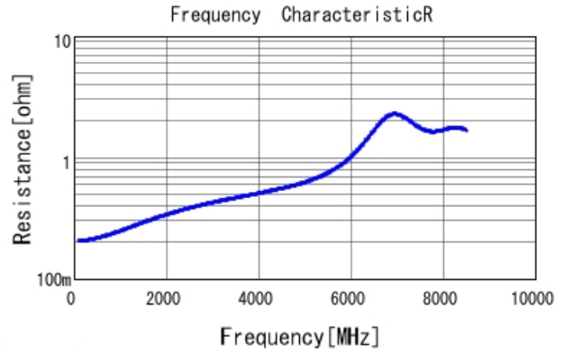
GRM1555C2A6R5WA01 R DCOV, 25degC
