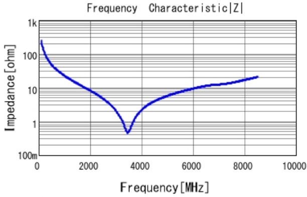
GRM1555C2A6R5WA01 |Z| DCOV, 25degC
