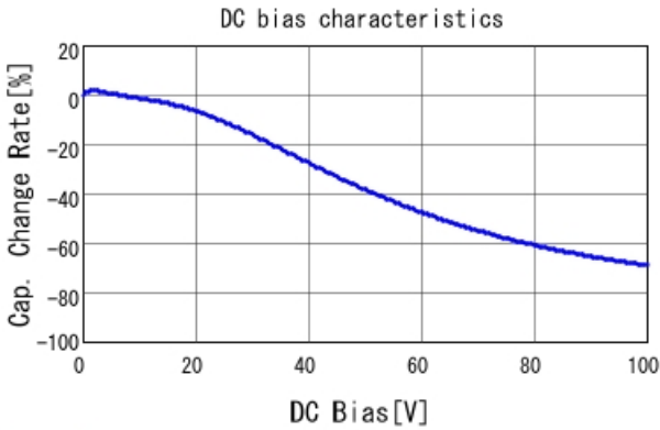
GRM31MR72A154KA01 C-DC bias capchange, 25.0degC, A
