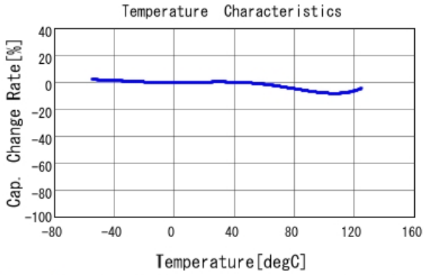
GRM31MR72A154KA01 C-Temp. capchange, DC0.0V, AC1.C
