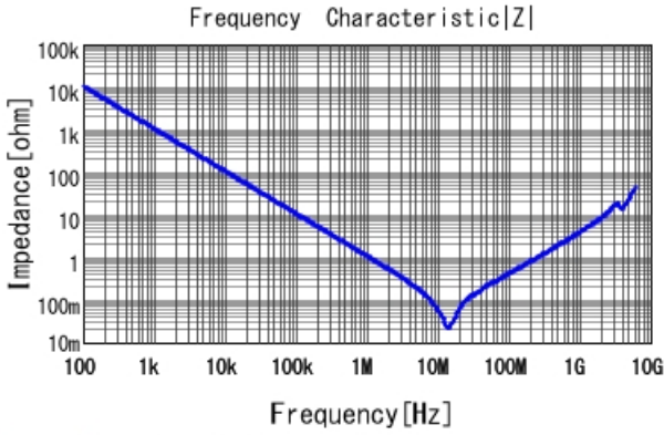
GRM31MR72A154KA01 |Z| DCOV, 25degC
