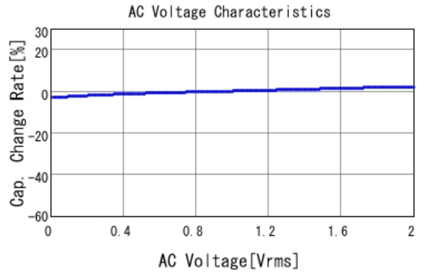
GRM31MR72A154KA01 C-AC Voltage capchange, DCOV, 25
