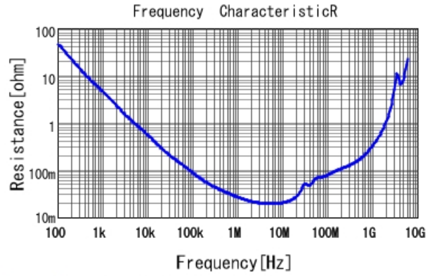
GRM31MR72A154KA01 R DCOV, 25degC
