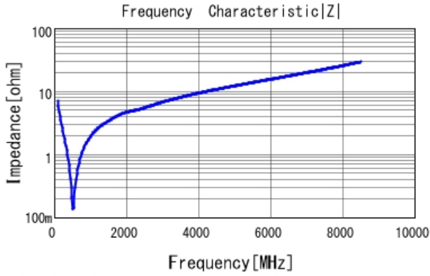
GCM1555C1H221JA16 |Z| DCOV, 25degC
