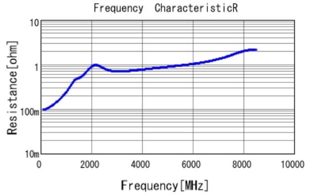
GCM1555C1H221JA16 R DCOV, 25degC
