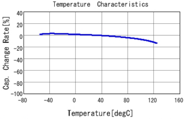
GRM32ER72A225MA35 C-Temp. capchange, DC0.0V, AC1.C
