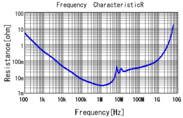
GRM32ER72A225MA35 R DCOV, 25degC
