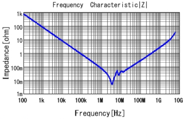
GRM32ER72A225MA35 |Z| DCOV, 25degC
