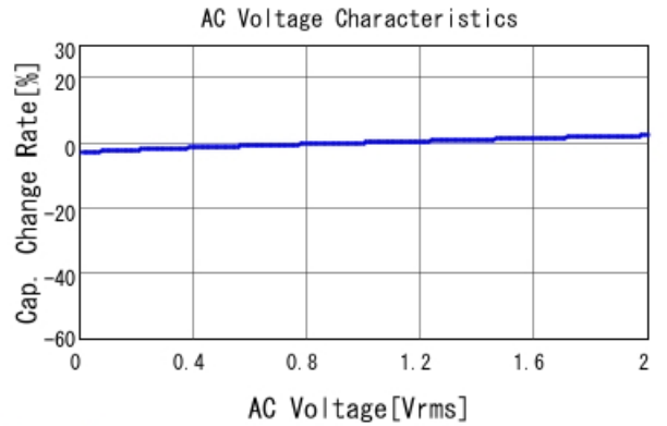
GRM32ER72A225MA35 C-AC Voltage capchange, DCOV, 25
