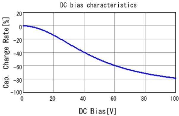
GRM32ER72A225MA35 C-DC bias capchange, 25.0degC, A
