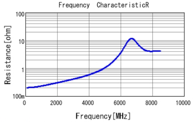
GRM1555C2A7R3WA01 R DCOV, 25degC
