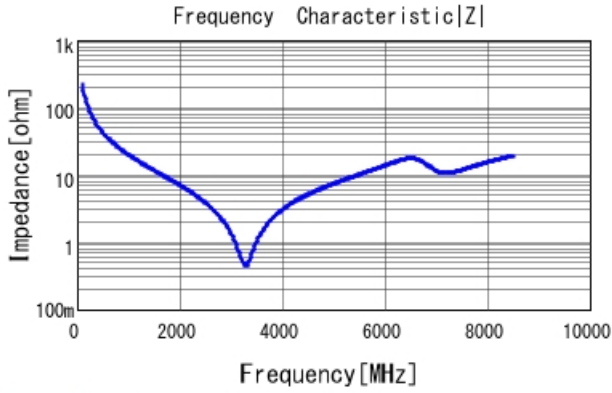
GRM1555C2A7R3WA01 |Z| DCOV, 25degC
