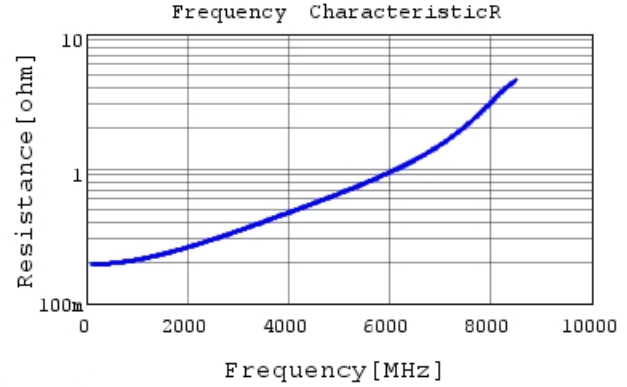
GRM0335C1H7R0DA01 R DCOV, 25degC
