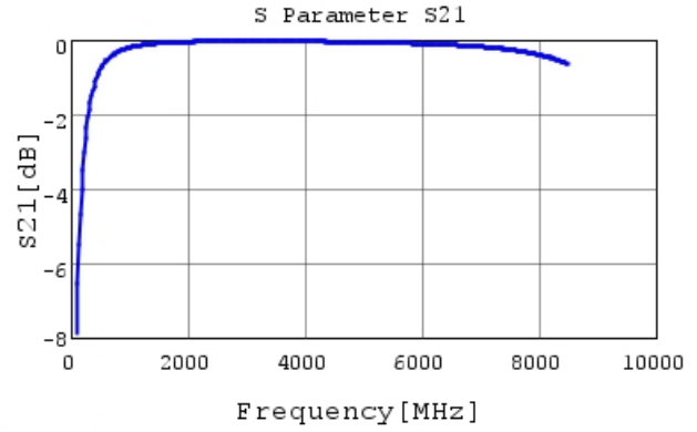
GRM0335C1H7R0DA01 S21 DCOV, 25degC
