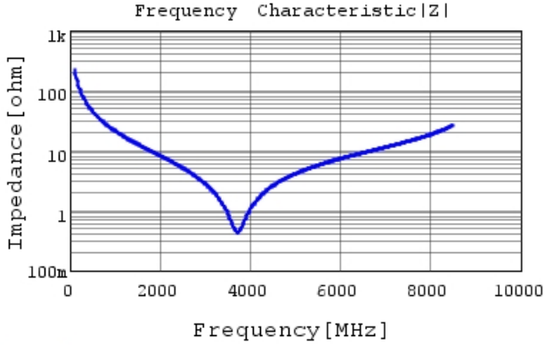
GRM0335C1H7R0DA01 |Z| DCOV, 25degC
