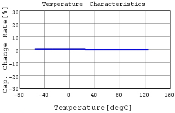
GRM0335C1H7R0DA01 C-Temp. capchange, DCOV, 1
