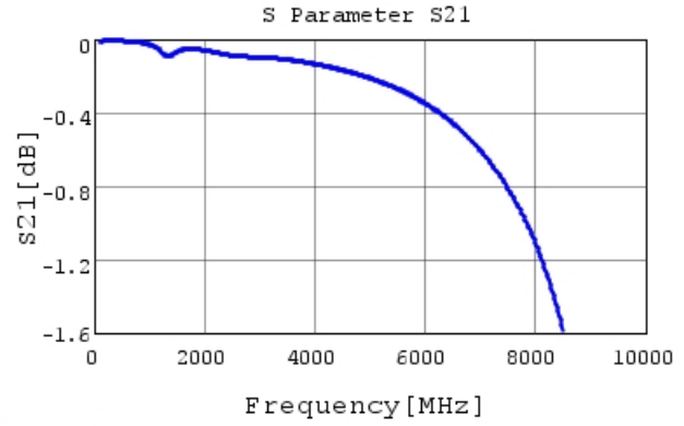
GCM1885C2A331JA16 S21 DCOV, 25degC
