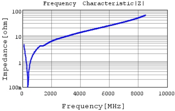
GCM1885C2A331JA16 |Z| DCOV, 25degC
