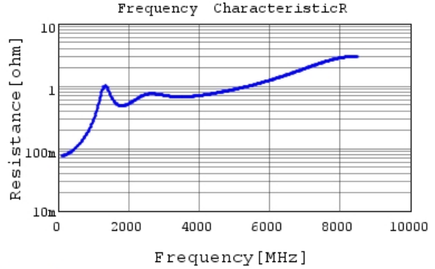
GCM1885C2A331JA16 R DCOV, 25degC
