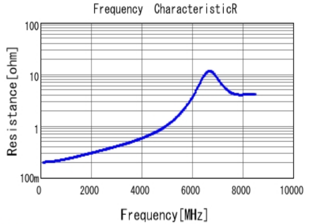
■ GRM1555C2A7R3CA01 R DCOV, 25degC
