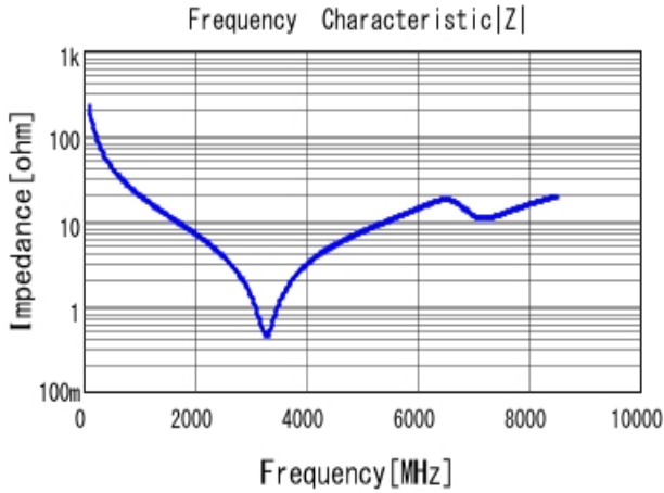
■ GRM1555C2A7R3CA01 |Z| DCOV, 25degC
