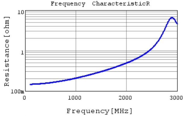
GRM31A5C3A390GW01 R DC0V, 25degC
