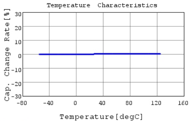
GRM31A5C3A390GW01 C-Temp. capchange, DC0V, 1
