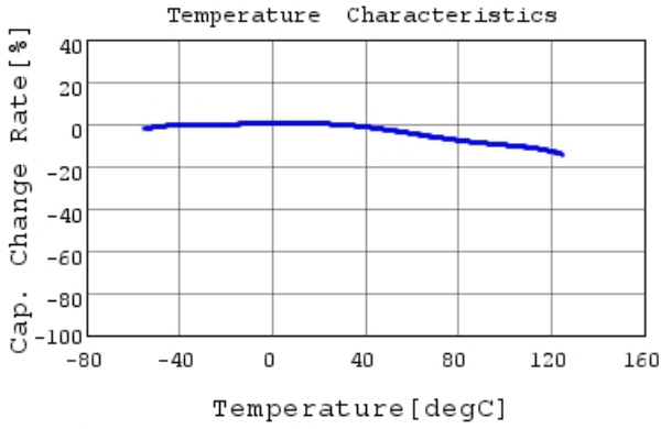
RCER71H475K3K1H03B C-Temp. capchange, DC0.0V
