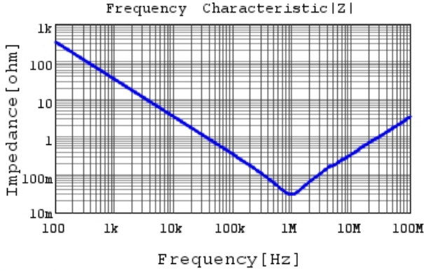
RCER71H475K3K1H03B |Z| DC0V, 25degC
