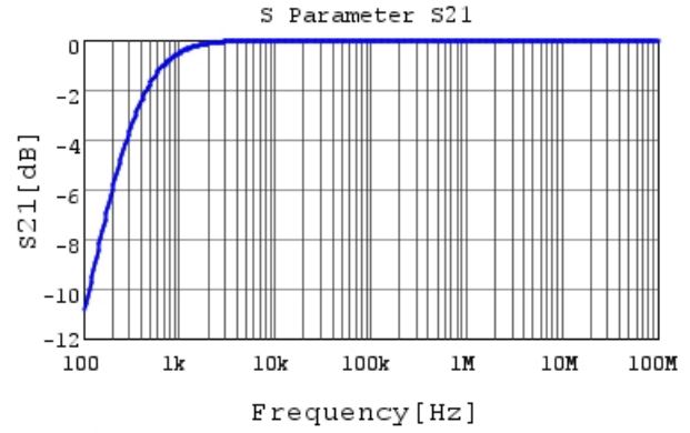
RCER71H475K3K1H03B S21 DC0V, 25degC
