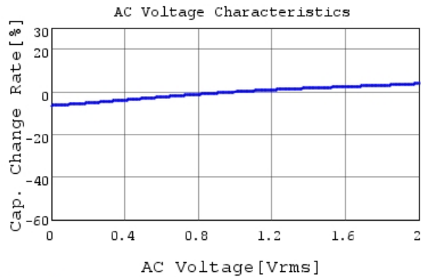
RCER71H475K3K1H03B C-AC Voltage capchange, I
