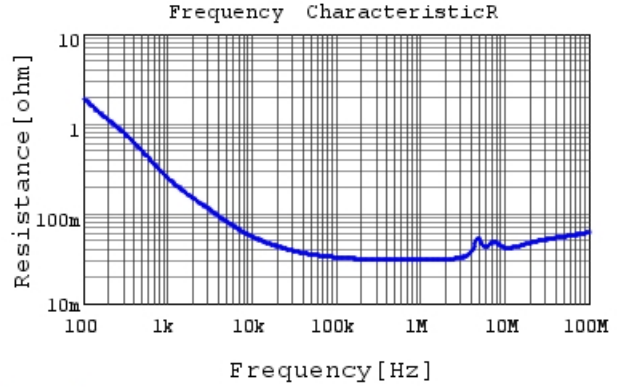
RCER71H475K3K1H03B R DC0V, 25degC
