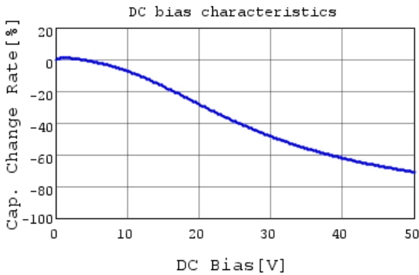
RCER71H475K3K1H03B C-DC bias capchange, 25.0
