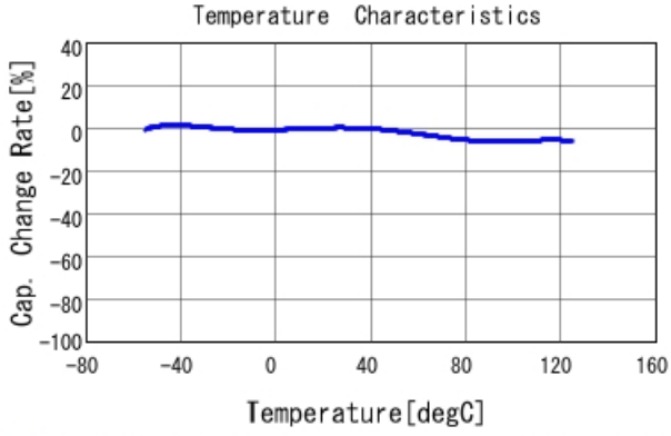
■ GCD188R72A272KA01 C-Temp. capchange, DCO. 0V, AC1. 0Vrm
