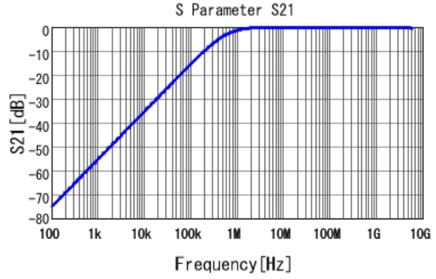
■ GCD188R72A272KA01 S21 DCOV, 25degC
