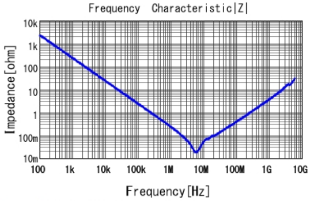
GCJ31CR71H684KA01 |Z| DCOV, 25degC
