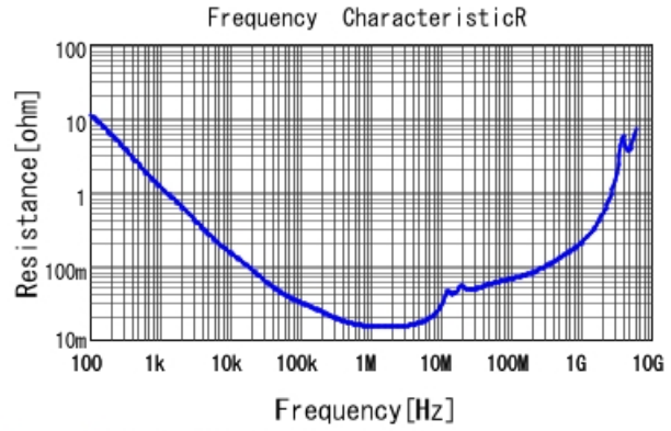
GCJ31CR71H684KA01 R DCOV, 25degC
