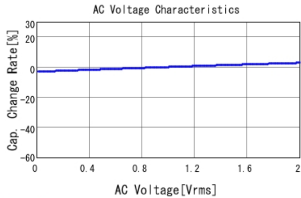
GCJ31CR71H684KA01 C-AC Voltage capchange, DCOV, 25
