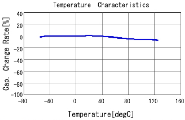
GCJ31CR71H684KA01 C-Temp. capchange, DC0.0V, AC1.C
