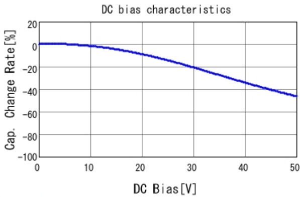
GCJ31CR71H684KA01 C-DC bias capchange, 25.0degC, A
