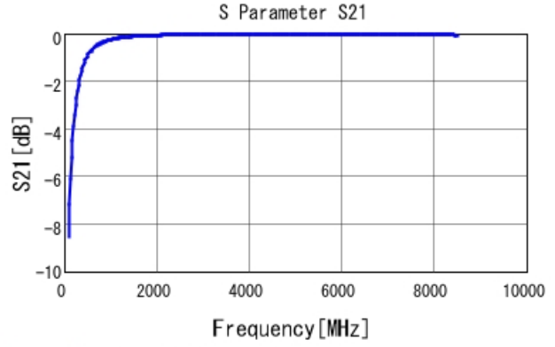
GRM0225C1E6R4WA03 S21 DCOV, 25degC
