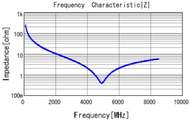
GRM0225C1E6R4WA03 |Z| DCOV, 25degC
