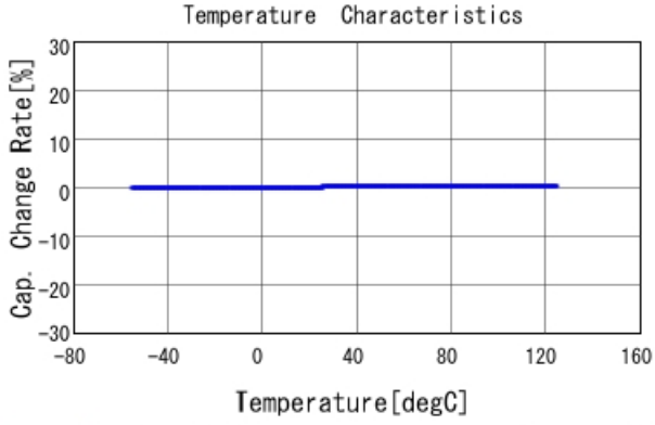
GRM0225C1E6R4WA03 C-Temp. capchange, DCOV, AC1Vrms
