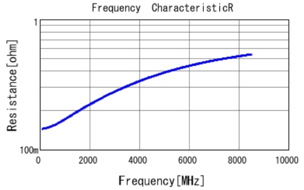
GRM0225C1E6R4WA03 R DCOV, 25degC
