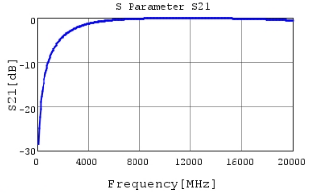
GRM0335C2AR60BA01 S21 DCOV, 25degC
