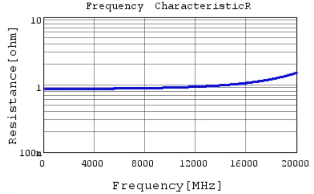
GRM0335C2AR60BA01 R DCOV, 25degC
