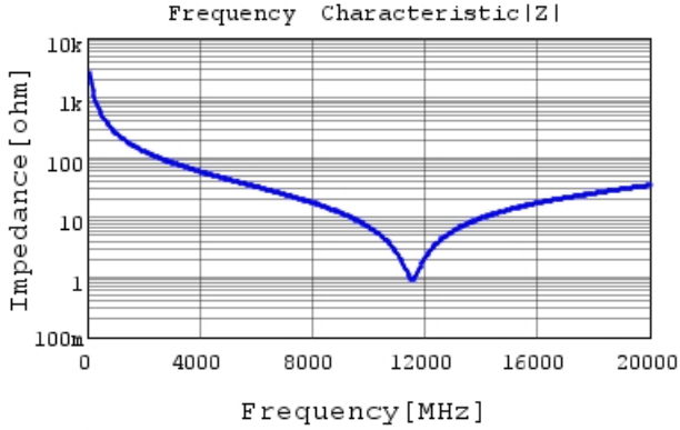
GRM0335C2AR60BA01 |Z| DCOV, 25degC
