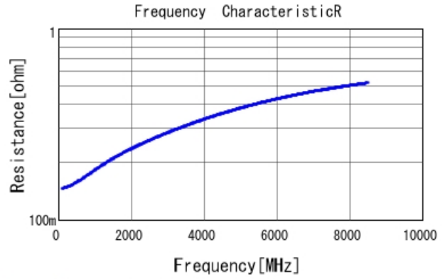
GRM0225C1E5R7DA03 R DCOV, 25degC
