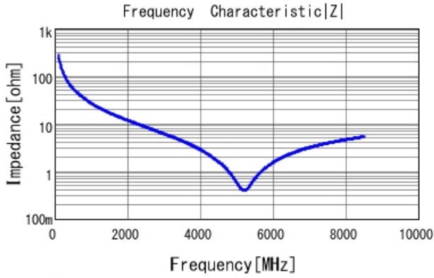
GRM0225C1E5R7DA03 |Z| DCOV, 25degC
