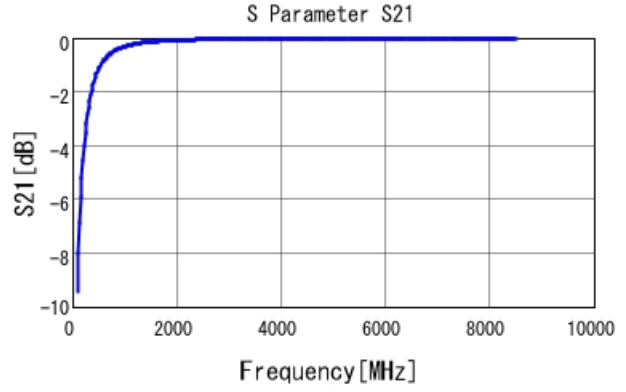
GRM0225C1E5R7DA03 S21 DC0V, 25degC
