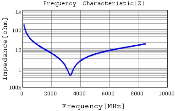
GRM0335C1H9R0DA01 |Z| DCOV, 25degC
