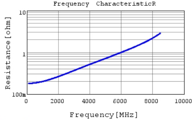
GRM0335C1H9R0DA01 R DCOV, 25degC
