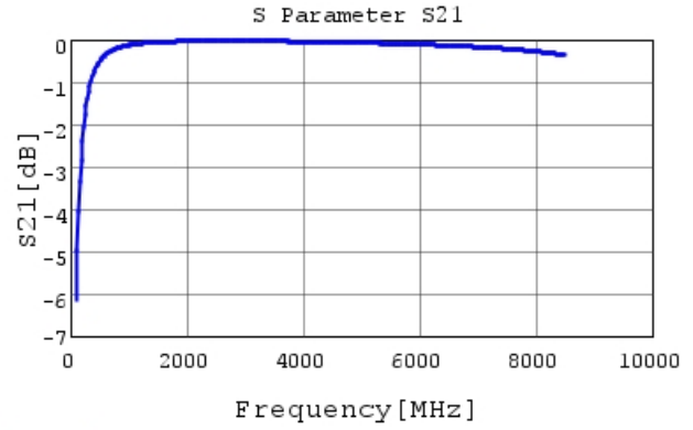
GRM0335C1H9R0DA01 S21 DCOV, 25degC
