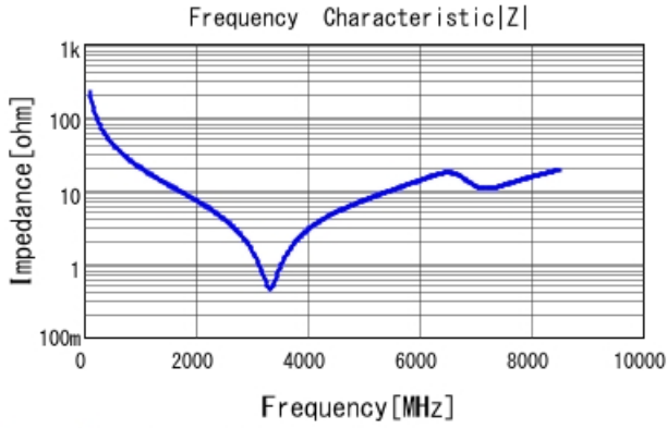
GRM1555C2A7R1DA01 |Z| DCOV, 25degC
