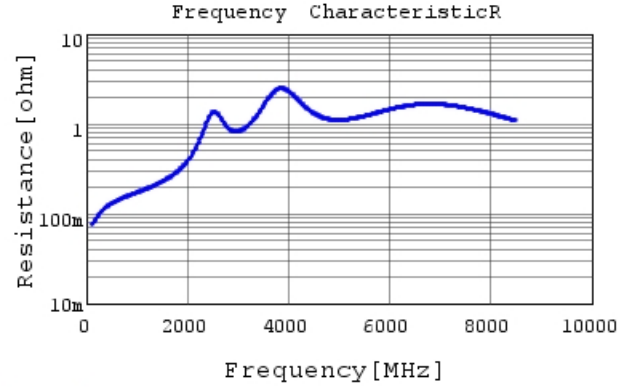
GCM1555C1H560JA16 R DC0V, 25degC
