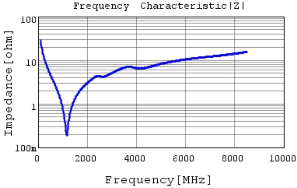
GCM1555C1H560JA16 |Z| DC0V, 25degC
