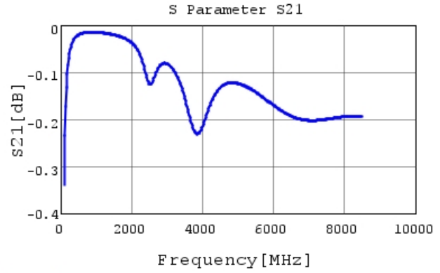
GCM1555C1H560JA16 S21 DCOV, 25degC
