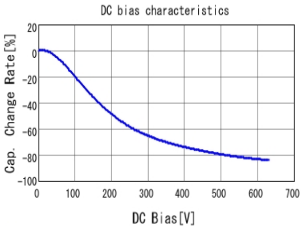
■ GCJ32DR72J333KXJ1 C-DC bias capchange, 25.0degC, AC1V
