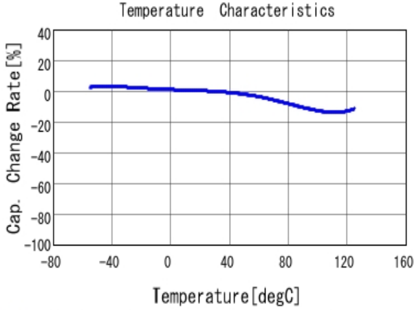
■ GCJ32DR72J333KXJ1 C-Temp. capchange, DCOV, AC1Vrms
