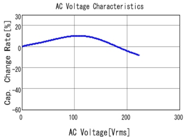
■ GCJ32DR72J333KXJ1 C-AC Voltage capchange, DC0V, 25.0d
