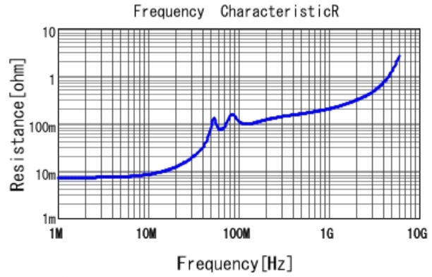
GRM3197U1H563JA01 R DCOV, 25degC
