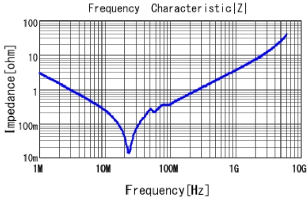
GRM3197U1H563JA01 |Z| DCOV, 25degC
