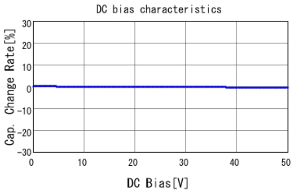
GRM3197U1H563JA01 C-DC bias capchange, 25.0degC, A
