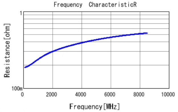
GRM0225C1E3R5BA03 R DCOV, 25degC
