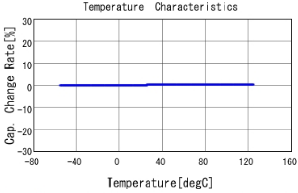
GRM0225C1E3R5BA03 C-Temp. capchange, DC0V, AC1Vrms
