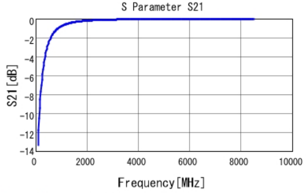
GRM0225C1E3R5BA03 S21 DC0V, 25degC
