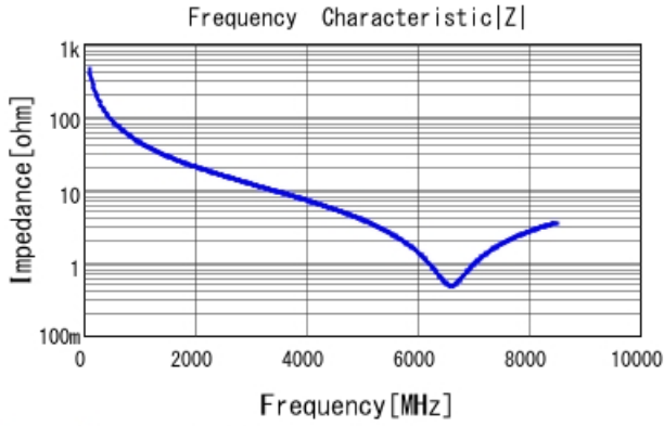
GRM0225C1E3R5BA03 |Z| DCOV, 25degC
