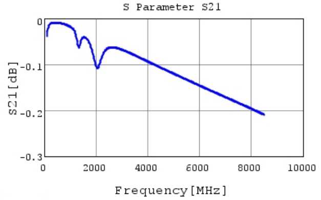
GCM1555G1H181JA16 S21 DCOV, 25degC
