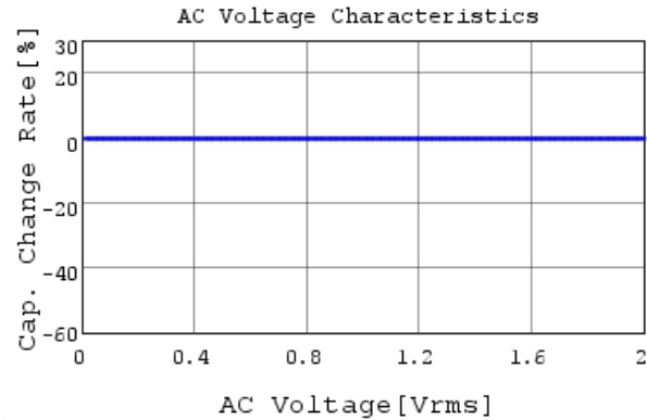
GCM1555G1H181JA16 C-AC Voltage capchange, DC
