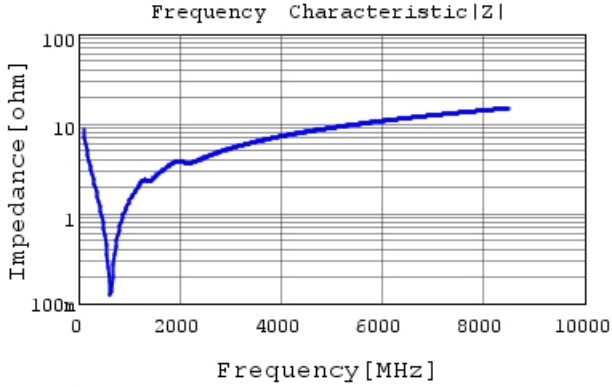
GCM1555G1H181JA16 |Z| DC0V, 25degC
