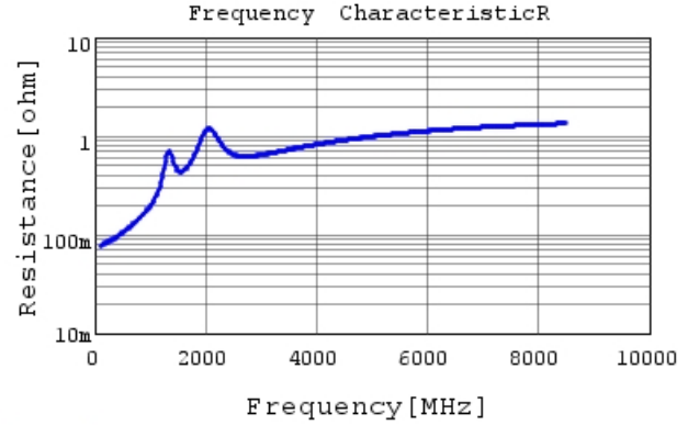
GCM1555G1H181JA16 R DC0V, 25degC
