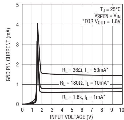
LT1965-1.8 GND Pin Current (Light Load)
