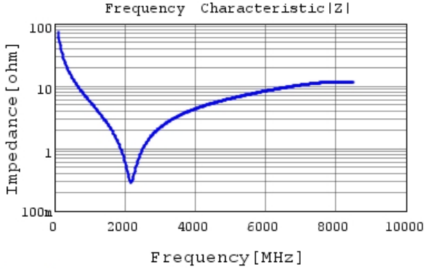
GRM0335C2A220JA01 |Z| DCOV, 25degC
