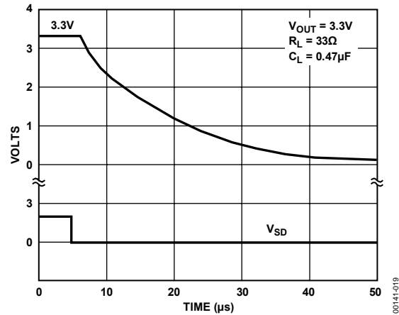
Figure 19. Turn-Off
