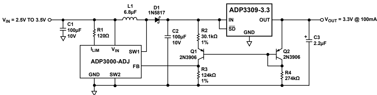
Figure 25. Constant Dropout Post Regulator
