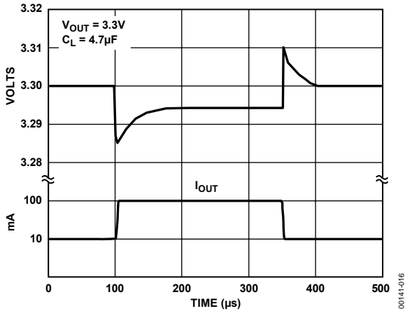
Figure 16. Load Transient
