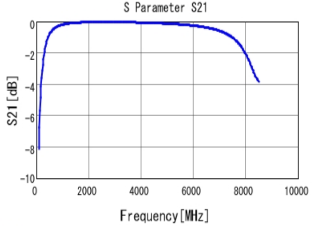
■ GRM1885C1H6R8BA01 S21 DCOV, 25degC
