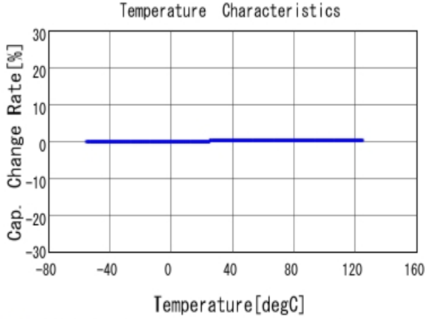
■ GRM1885C1H6R8BA01 C-Temp. capchange, DCOV, AC1Vrms
