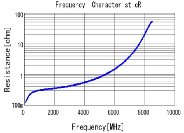
■ GRM1885C1H6R8BA01 R DCOV, 25degC
