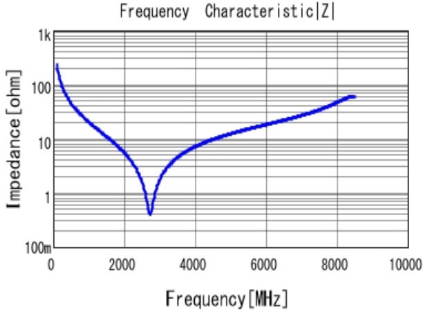
■ GRM1885C1H6R8BA01 |Z| DCOV, 25degC
