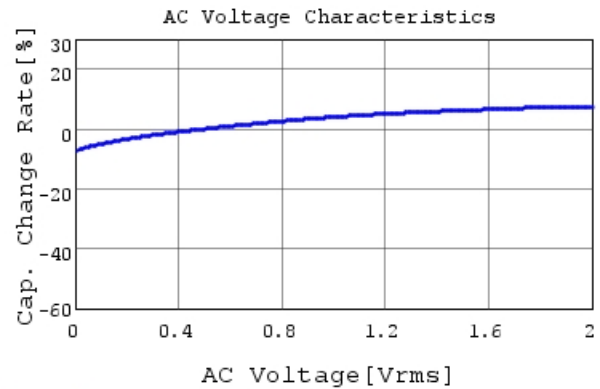
GRM033C80J223ME01 C-AC Voltage capchange, Dc
