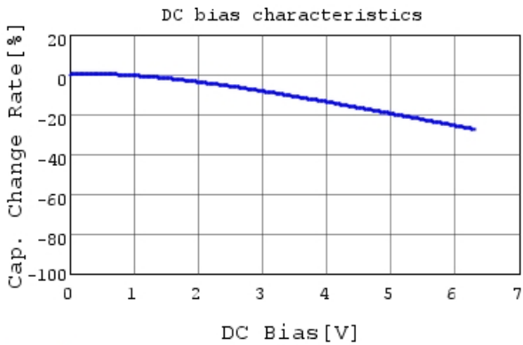
GRM033C80J223ME01 C-DC bias capchange, 25.0c
