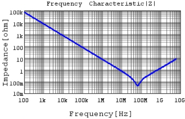
GRM033C80J223ME01 |Z| DCOV, 25degC
