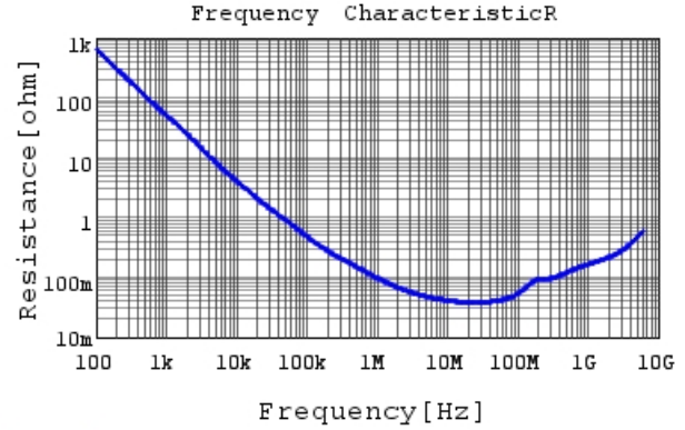
GRM033C80J223ME01 R DCOV, 25degC
