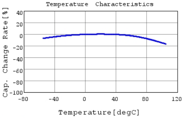
GRM033C80J223ME01 C-Temp. capchange, DC0.0V,
