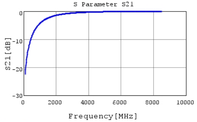
GJM0335C1E1R2CB01 S21 DCOV, 25degC
