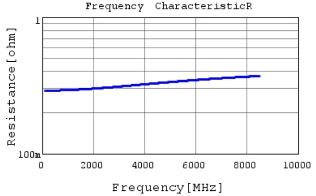
GJM0335C1E1R2CB01 R DCOV, 25degC
