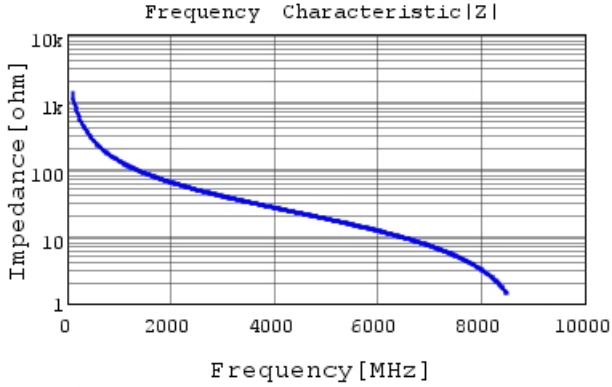
GJM0335C1E1R2CB01 |Z| DCOV, 25degC
