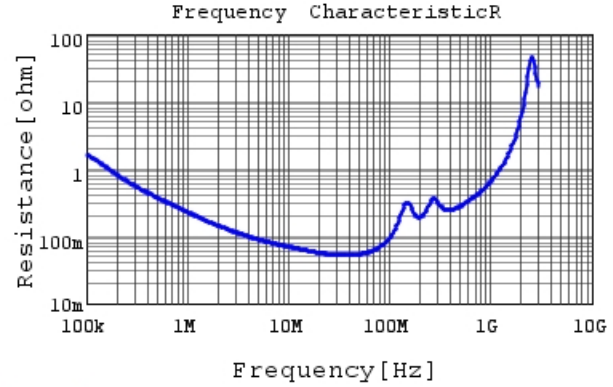
GR455DR73D103KW01 R DCOV, 25degC
