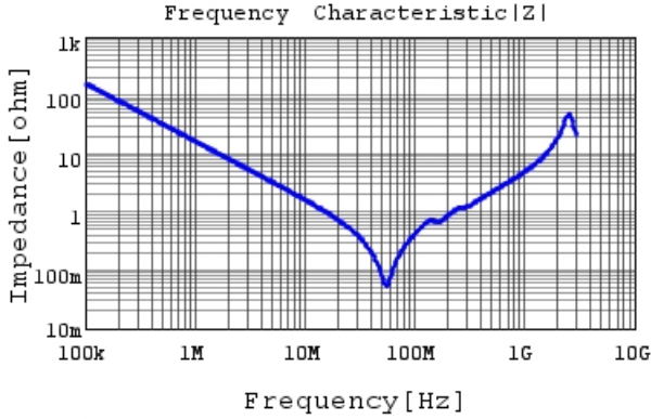
GR455DR73D103KW01 |Z| DCOV, 25degC
