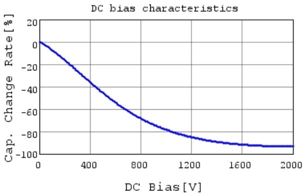
GR455DR73D103KW01 C-DC bias capchange, 25.0c
