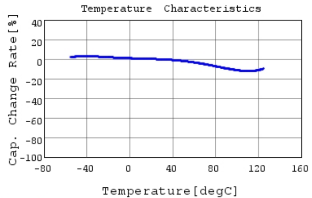
GR455DR73D103KW01 C-Temp. capchange, DCOV, 1
