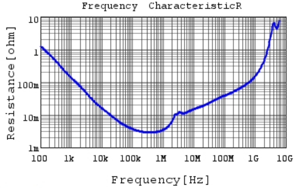
GRT31CC81C226KE01 R DCOV,25degC
