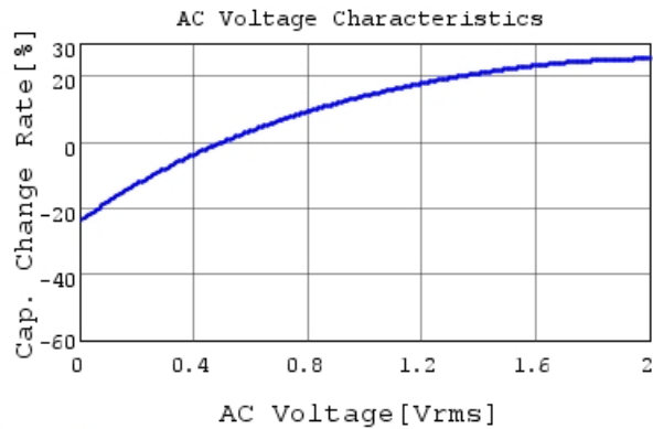
GRT31CC81C226KE01 C-AC Voltage capchange, Dc
