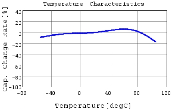
GRT31CC81C226KE01 C-Temp. capchange, DC0.0V,
