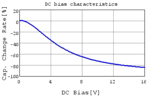
GRT31CC81C226KE01 C-DC bias capchange, 25.0c
