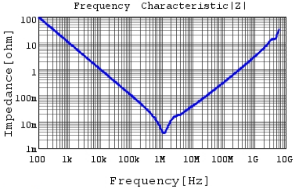
GRT31CC81C226KE01 |Z| DCOV,25degC
